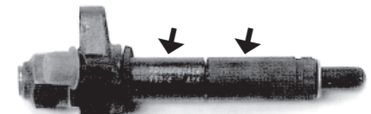
AKF/KBL Injector AKF Core Class 224 KBL Core Class 227
